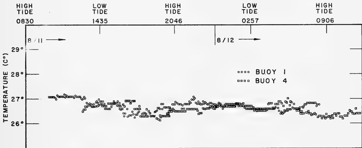
Figure 4. Temperature records for the second day, Buoys 1 and 4, at 170 ft.
